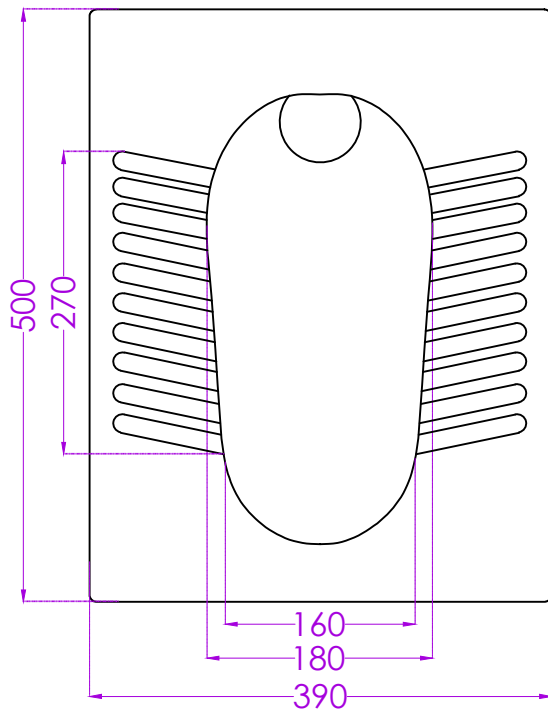
PLAN
